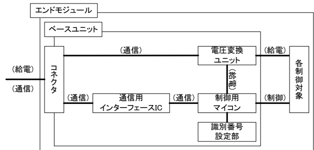
Figure 3: Common controller of modules
